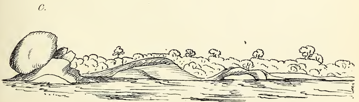
Forms of Granite rocks.
